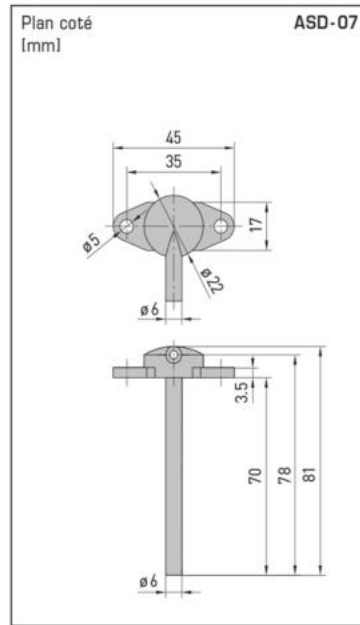
ASD-07 Embouts de raccordement
