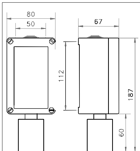
Fig. 1 Dimensioni/Size/Dimensions
