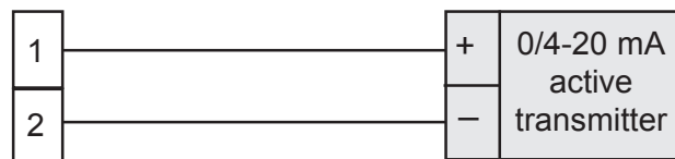
Fig. 10- 0/4-20 mA input wiring for active transmitter
